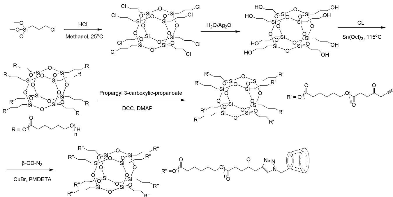
Scheme 1. Synthesis of POSS-PCL-β-CD star-shaped copolymer by the combination of ROP and click chemistry.
