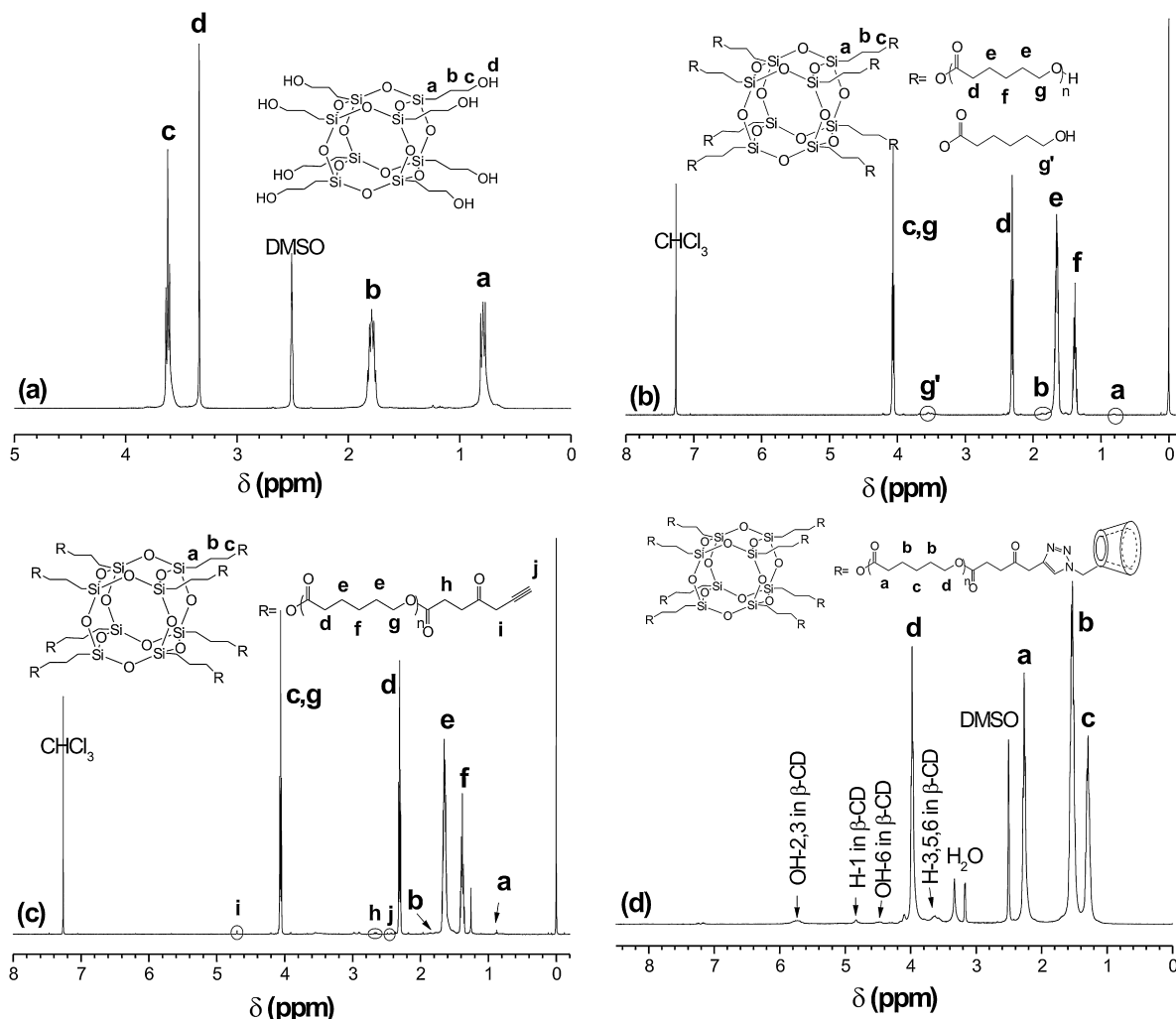
Fig. 1. ^1\text{H} NMR spectra of (a) POSS-OH, (b) POSS-PCL, (c) alkynyl POSS-PCL, and (d) POSS-PCL- \beta -CD.
